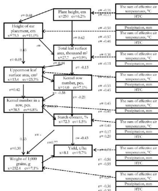
Figure 1: Model of the influence of weather conditions on the formation of phenotypic productivity of early corn hybrids
