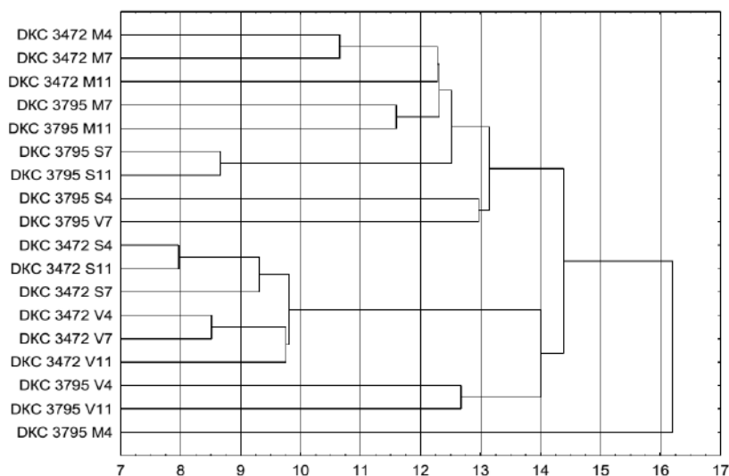
Figure 5: Clustering of medium-early maize hybrids by a set of economically valuable traits, by studying the influence of fraction and depth of seed wrapping
