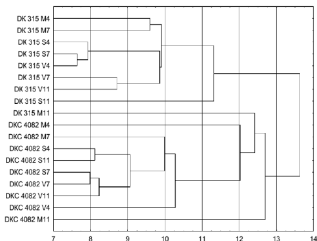
Figure 6: Clustering of medium-ripe corn hybrids by a set of economically valuable traits, by studying the influence of fraction and depth of seed wrapping
