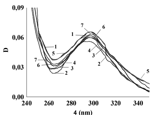
Fig. 8. UV spectra of cisplatin in 0.9 % NaCl solution at different pH: 1 – 3.6; 2 – 4.6; 3 – 5.6; 4 – 6.6; 5 – 7.6; 6 – 8.6; 7 – 9.6
