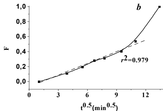
Fig. 10. Experimental kinetic dependences of Cisplatin adsorption in the coordinates -\ln(1-F) - t (a) and F - t^{0.5} (b)
