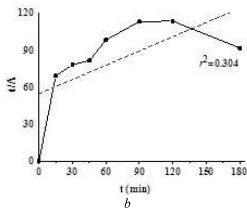
Fig. 12. Kinetic dependences of Cisplatin adsorption in the coordinates of the pseudo-first order model (a) and the pseudo-second order model (b)
