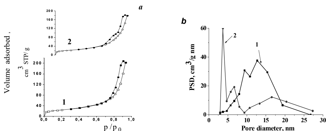
Fig. 6. Adsorption/desorption isotherms (a) and pore distribution (b) of samples: 1 – \text{Fe}_3\text{O}_4 , 2 – \text{Fe}_3\text{O}_4/\text{Al}_2\text{O}_3/\text{C}
