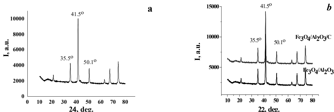
Fig. 1. XRD patterns of NPs of the original \text{Fe}_3\text{O}_4 (a); NCs \text{Fe}_3\text{O}_4/\text{Al}_2\text{O}_3 and \text{Fe}_3\text{O}_4/\text{Al}_2\text{O}_3/\text{C} (b)
